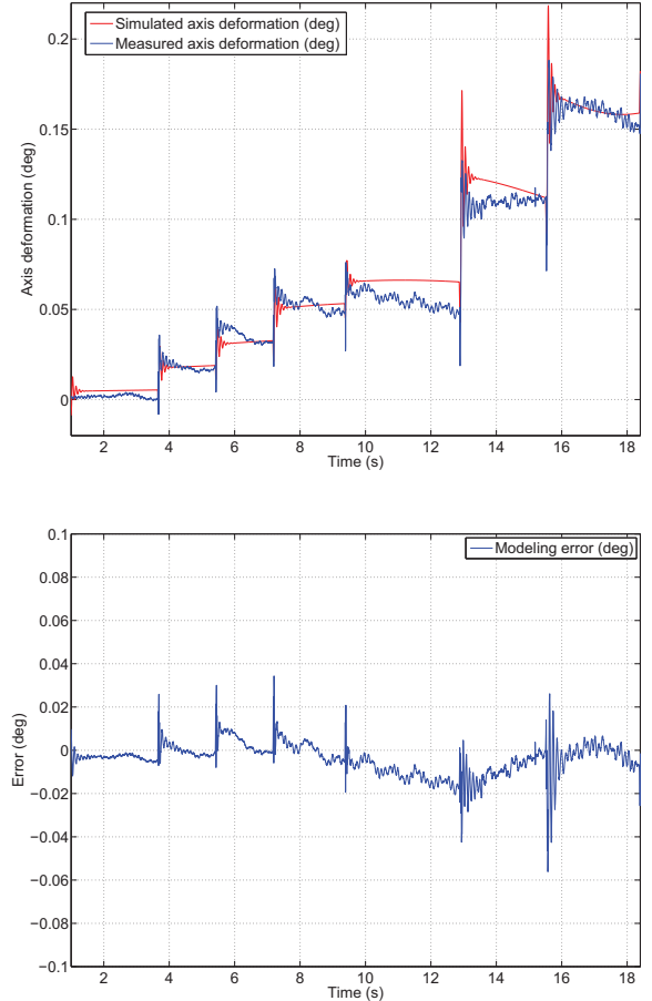
Fig. 12. Axis deformation model validation (upper) and modeling error (below)
