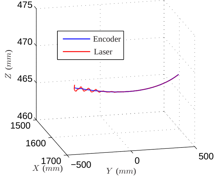
Fig. 3. Experimental measurement of the robot trajectory tracking in the (X, Y, Z) cartesian frame.
