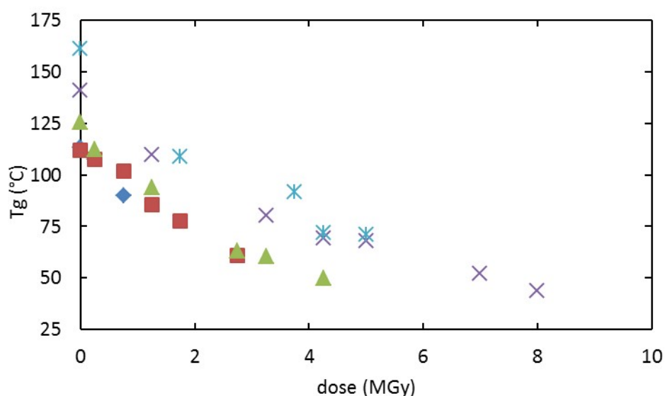
Figure 3. Glass transition temperature of irradiated networks B( \blacklozenge ), C( \blacksquare ), D( \blacktriangle ), F( \times ) and G( * ).
