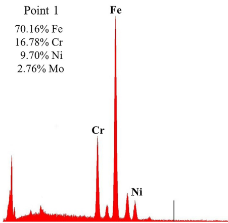
Fig. 17. Chemical composition at point 1 (Fig. 14).
