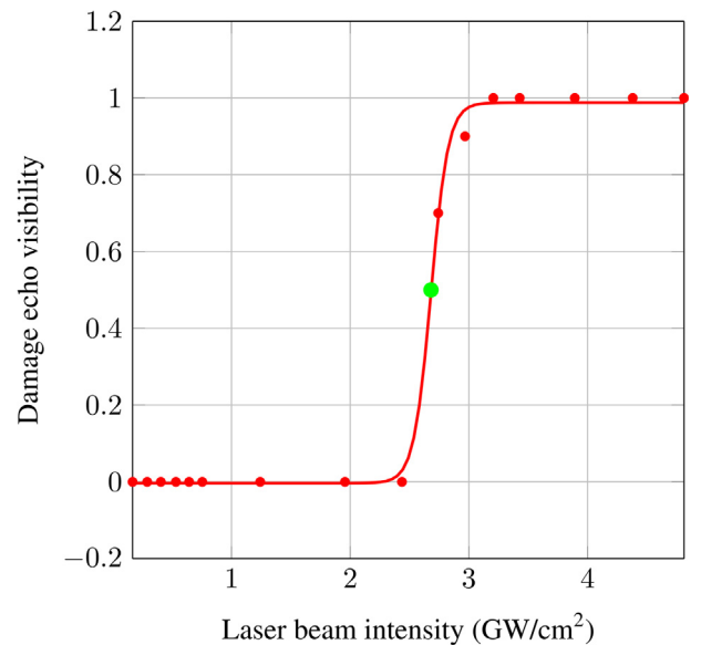
Fig. 9. Damage echo visibility as function of laser beam intensity: Damage threshold in the case of one laser pulse.
