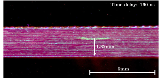
Fig. 13. Damage depth in the case of symmetrical laser shock configuration and 160 ns time delay.
