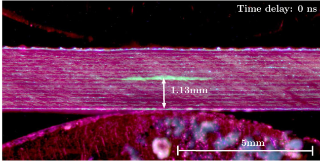
Fig. 11. Damage depth in the case of symmetrical laser shock configuration and zero time delay.
