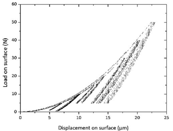
FIG. 10. Multicycle macro-indentation performed on the BK7 glass sample with 5 cycles performed at constant loads between 5 and 50 N.
