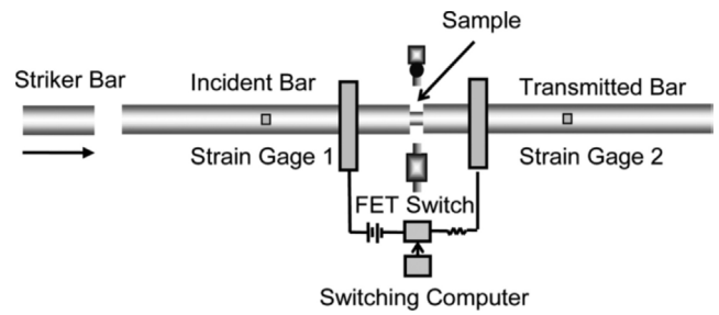
Fig. 7. Schematic of the NIST electrical pulse-heated Kolsky bar setup [39].
