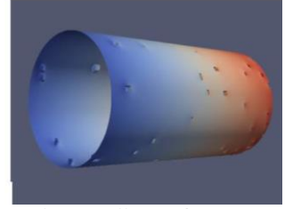
Fig. 3. Visual illustration of adsorbed particles for two different Péclet numbers after the injection of 3000 particles (A) Pe=0.0015 and (B) Pe=150 .
