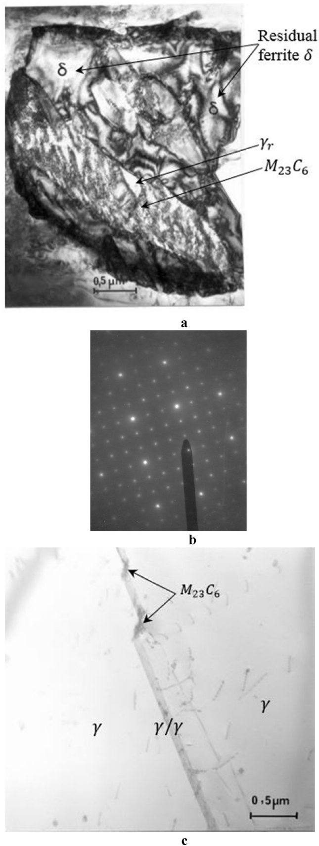
Fig. 5. Decomposition of \delta ferrite after aging at 550 °C during 10 000 h (TEM examination): (a) Decomposition of \delta ferrite into M_{23}C_6 and regenerated austenite ( \gamma_r ); (b) SAD of M_{23}C_6 carbide and regenerated austenite ( \gamma_r ); (c) Nucleation of M_{23}C_6 carbide at the austenite grain boundaries.
