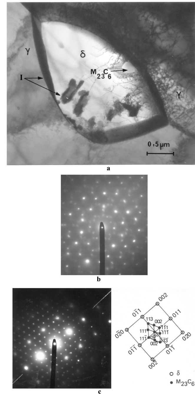
Fig. 4. Decomposition of \delta ferrite after aging at 550 °C during 1000 h (TEM examination): (a) F.K phase (I phase) and M_{23}C_6 carbide at the \delta/\gamma interface; (b) SAD of F.K phase and \delta ferrite matrix; (c) SAD of M_{23}C_6 carbide and \delta ferrite matrix.
