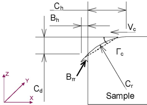
Fig. 9. Burr with chamfer and its geometrical descriptors.
