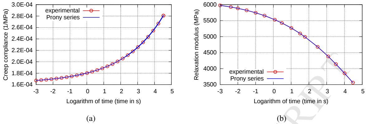
Figure 6: Evolution with time of (a) the creep compliance for the \text{CaCO}_3 -filled polyester of Jerina et al. (1982), (b) the relaxation modulus of the same material, computed with the procedure described in the Appendix I of Park and Kim (1999). The figures also illustrate the numerical simulation using Prony series (material parameters are provided in Table 2, columns 3 and 4).
