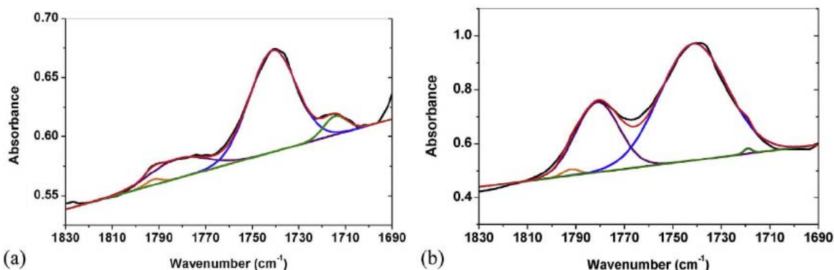
Fig. 2. Deconvolution of the region of C=O bonds in the IR spectrum of PEEK after 324 h of exposure at 300 °C under 0.21 bar of oxygen (a) and after 196 h of exposure at 250 °C under 10 bars of oxygen (b).
