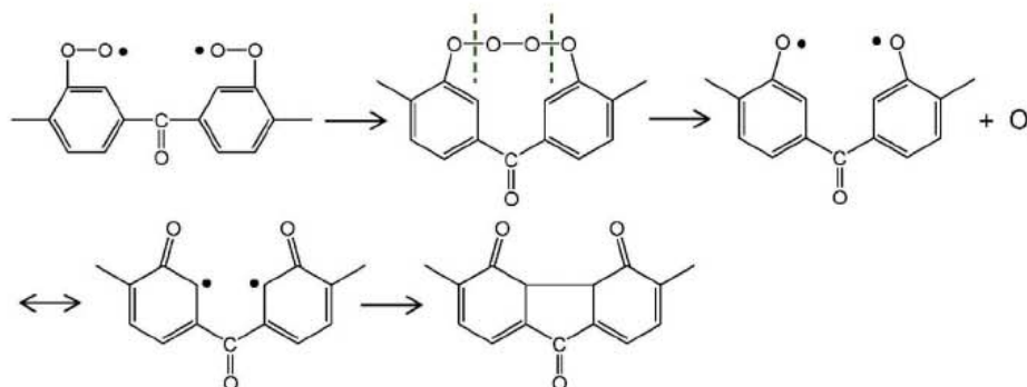
Fig. 16. Formation mechanism of fluorenone by intramolecular coupling of peroxy radicals.
