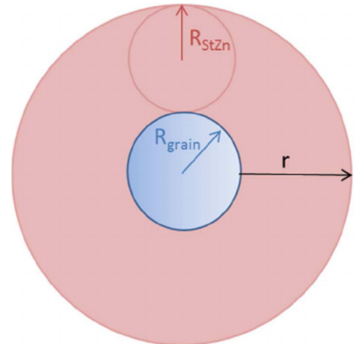
Fig. 1. "Embedded grain" configuration in the 3DiP software used to calculate the mean dose rate deposited by a grain of PuO 2 in a grain of zinc stearate with a radius R_{\text{StZn}} .
