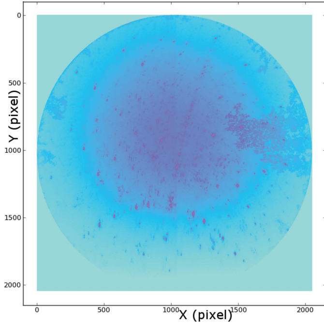
Figure 7 μLaue diffraction pattern of the sample, showing peaks from numerous \text{ZrO}_2 crystals. The splitting of a number of diffraction spots is due to the contribution of many different small crystals having slightly different orientations (within less than 0.5^\circ of one another). A close-up is shown in Fig. 9.
