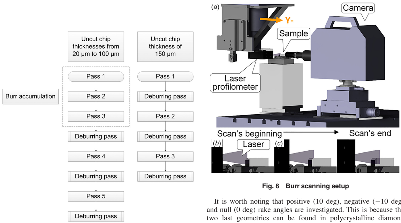
Fig. 7 Experimental sequence of cutting tests
