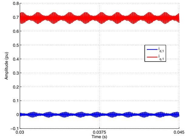
(a) Main Machine d_1 and q_1 currents
