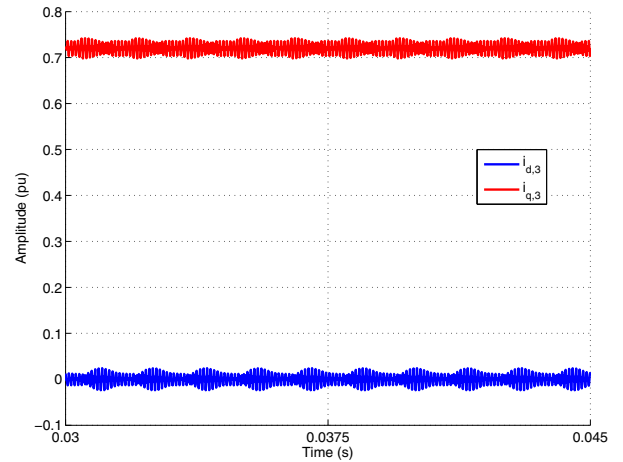
(b) Secondary Machine d_3 and q_3 currents
