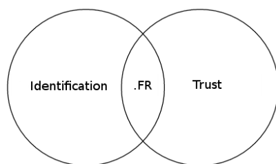
Figure 2. Identification-Trust link [12]
