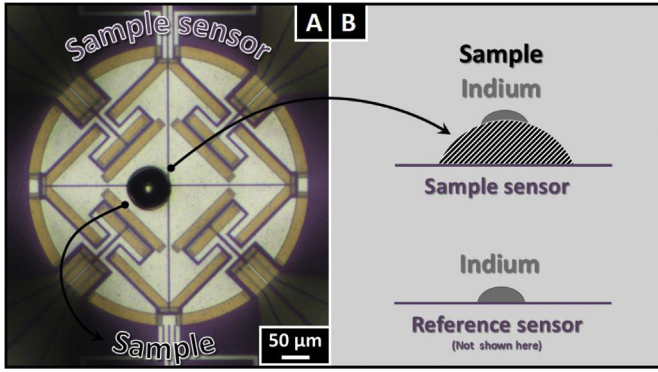
Fig. 2. (A) Photography of the sample sensor. (B) Schematic representation of the positioning of both sample and indium on sample and reference sensors for the determination of the static thermal lag.
