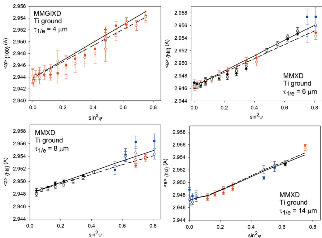
Figure 10 Similar results to those in Fig. 9, but for a ground Ti sample (the same legend and convention of data presentation apply).
