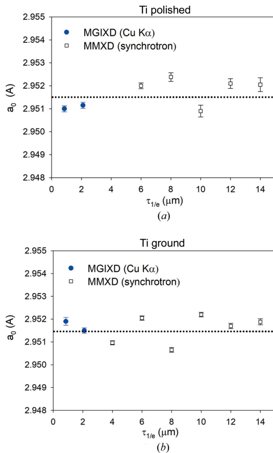
Figure 12 The depth-dependent profile (in the range 0–14 \mu\text{m} ) of lattice parameter a_0 for (a) polished and (b) ground samples. Comparison of the results from a classical diffractometer (MGIXD) and synchrotron EDDI experiment (MMXD).
