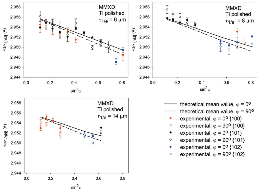
Figure 9 Example of \langle a(\phi, \psi) \rangle_{\{hkl\}} versus \sin^2\psi plots obtained using multireflection analysis for a polished Ti sample. The lines represent mean values of theoretical \langle a(\phi, \psi) \rangle_{\{hkl\}} parameters over all available reflections, while the experimental data are shown using different colours for different hkl reflections.
