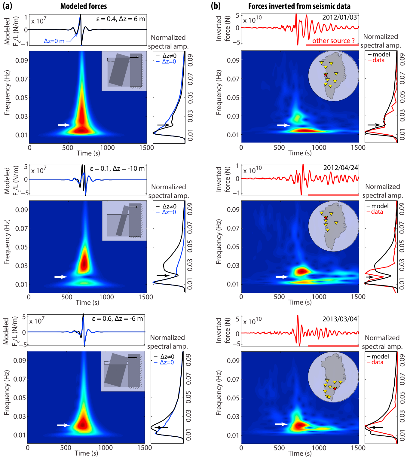
Figure 12. Comparison of the forces (a) simulated with iceberg capsize models and (b) inverted from seismic data, both filtered between 0.01 and 0.1 Hz, as well as the associated normalized spectrograms and power spectra. These simulated and inverted forces are for systems out of buoyant equilibrium (i.e., \Delta z \neq 0 ). For field data in Greenland (column (b)), locations of the calving events and GLISN stations used in the waveform inversion are indicated on inset maps by red stars and yellow triangles, respectively. The power spectra panels show the forces inverted from seismic data (red curves), modeled with either submarine or subaerial icebergs (black curves), and modeled with neutral icebergs (blue curves). The comparison between models and data show that seismic data spectral peaks or gaps indicated by arrows can be explained by the initial buoyant state of the capsizing icebergs, especially when they are out of their flotation level when they start calving.
