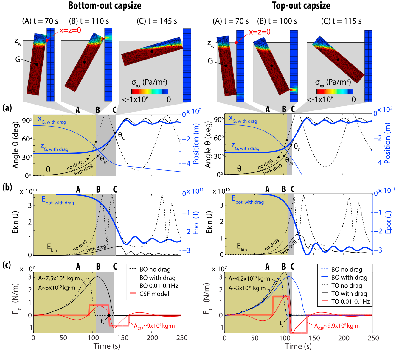
Figure 4. Results of bottom-out (left) and top-out (right) capsize simulations for an iceberg with \epsilon = 0.2 and H = 800 m. Top images illustrate capsize motions at different time steps: (A) when the iceberg is accelerating, (B) when the contact force with the wall is maximum, and (C) when at the loss of the iceberg-wall contact. The color scale represents the stress component \sigma_{xx} and is saturated beyond -1 \times 10^6 Pa, to simplify the illustration. Variations with time of (a) angle of rotation ( \theta , black curve) and coordinates x_G and z_G of the center of mass G (blue), (b) iceberg kinetic ( E_{kin} , black) and potential ( E_{pot} , blue) energies, and (c) horizontal force density ( F_c , black) and corresponding 0.01-0.1 Hz band-pass filtered force (red). The red thick curve shows the CSF model that best fits the force in the seismic band. In each graph, dashed curves represent time series of \theta , E_{kin} and F_c when water drag is not accounted for. Gray-shaded boxes indicate the time range when the iceberg is in contact with the wall (i.e., F_c > 0 N and \theta \leq \theta_C ). Same for yellow boxes but for capsize simulations without drag. \theta_M and \theta_C in (a) indicate the angles for maximum contact force and loss of iceberg/wall contact, respectively.
