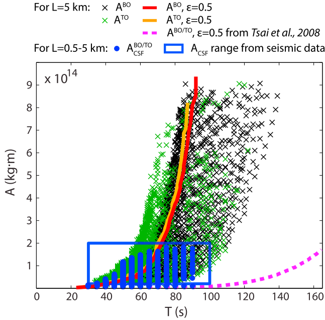
Figure 5. Force magnitudes A (kg·m) versus durations T' which corresponds to the effective duration of the force. Crosses are for BO (black) and TO (green) capsizes with iceberg height H = 100 – 1,000 m, aspect ratio \epsilon = 0.1 – 0.7 and length L = 5,000 m. Red and orange curves are for the specific value \epsilon = 0.5 , for BO and TO, respectively. The pink dashed curve indicates the results of Tsai et al. (2008) for the same iceberg dimensions, BO and TO together. Blue points are CSF magnitudes A_{CSF} computed by integrating twice the CSF models that fit the 0.01- to 0.1-Hz filtered forces generated by BO and TO capsizes of icebergs with lengths varying between 500 and 5,000 m. Computed A_{CSF} values are in the range of seismic observations (blue box) derived from glacial earthquake CSF inversions (Tsai & Ekström, 2007; Veitch & Nettles, 2012).
