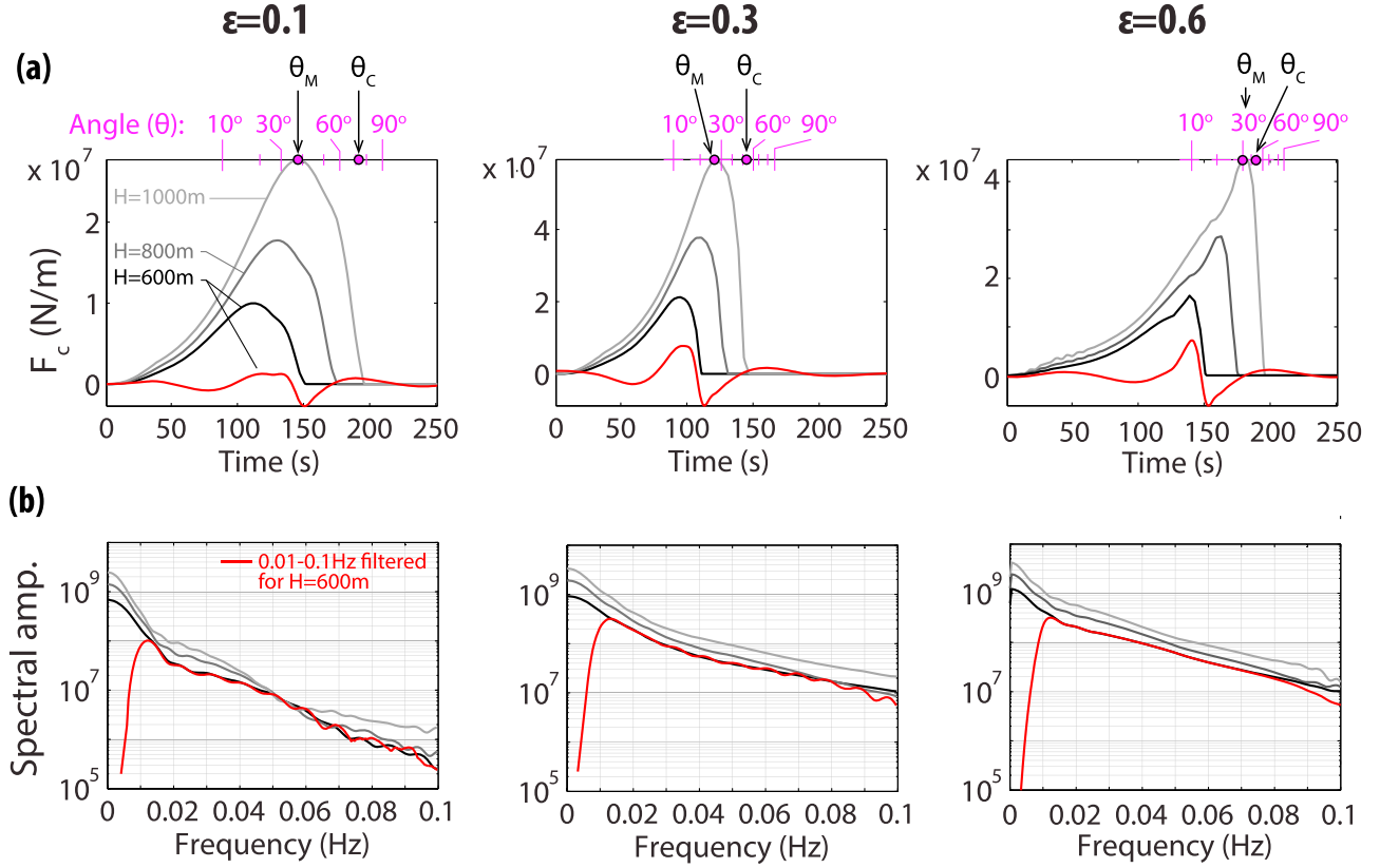
Figure 7. (a) Variations of the force history for three BO iceberg heights H = 600, 800 , and 1,000 m, and aspect ratios \epsilon = 0.1, 0.3 , and 0.6 . The red curves show the 0.01- to 0.1-Hz filtered forces for H = 600 m. The rotation angle \theta for 1,000-m-high iceberg capsizes are indicated in purple at the top of each panel. (b) Variations of spectral amplitudes with frequency, associated with each modeled force.
