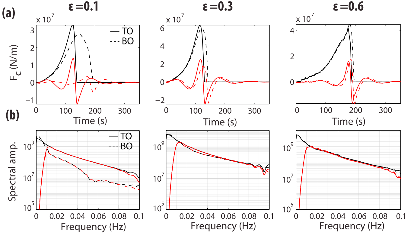
Figure 9. (a) Variations of the force history for TO (solid curves) and BO (dashed curves) iceberg capsizes with \epsilon = 0.1, 0.3 and 0.6 and H = 1000 m. The red curves show the 0.01- to 0.1-Hz filtered forces. (b) Variations of spectral amplitudes with frequency, associated with each force model.
