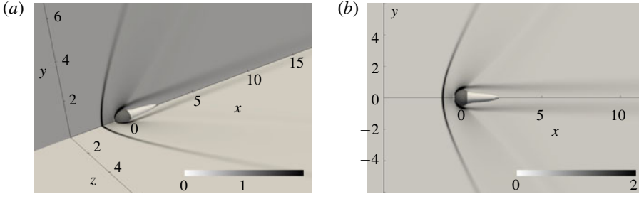
FIGURE 13. Schlieren-like visualization of the base flow at Re = 280 and M = 1.2 . Contours of the density gradient on (a) the two perpendicular x - y and x - z planes and (b) a 2-D view on the x - y plane.
