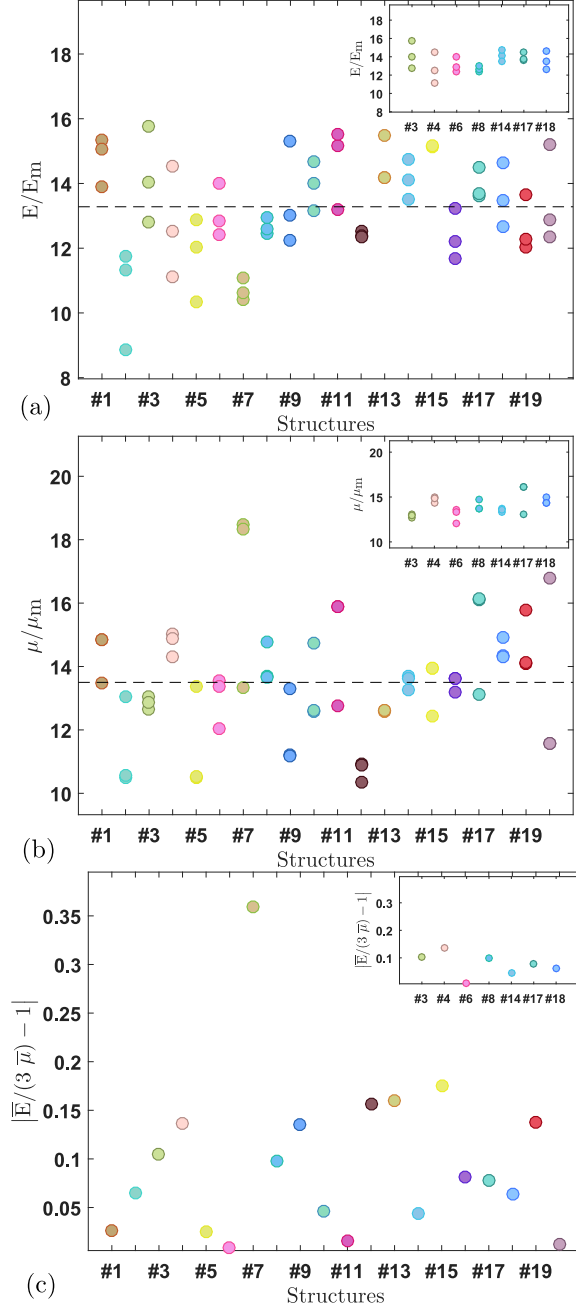
Figure 6: Values of the Young modulus (a) and shear modulus (b) obtained in the directions of the three cell axes and normalized by the matrix values for 20 microstructures. Isotropy criterion (c) calculated with the average Young modulus and average shear modulus for each microstructure. Insets correspond to the same data but considering only the 7 selected microstructures
