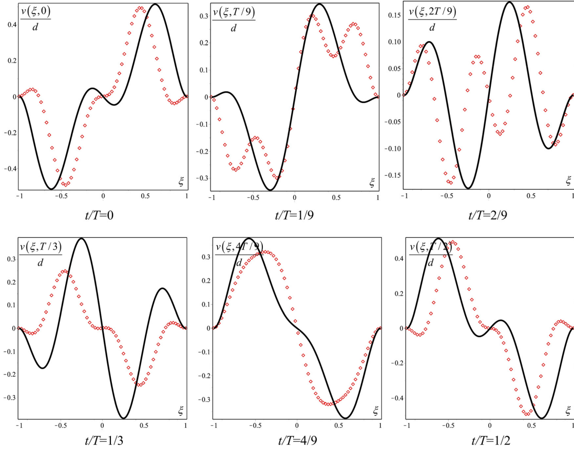
Fig. 7 Shapes assumed by local (—) and nonlocal ( \diamond , e_0 a = 2 nm, \zeta = 0.04 ) CNTs when \omega/\omega_2 = 1.163 and V_1/d \approx 0.33 , point P_1 in Fig. 5, along half a vibration cycle
