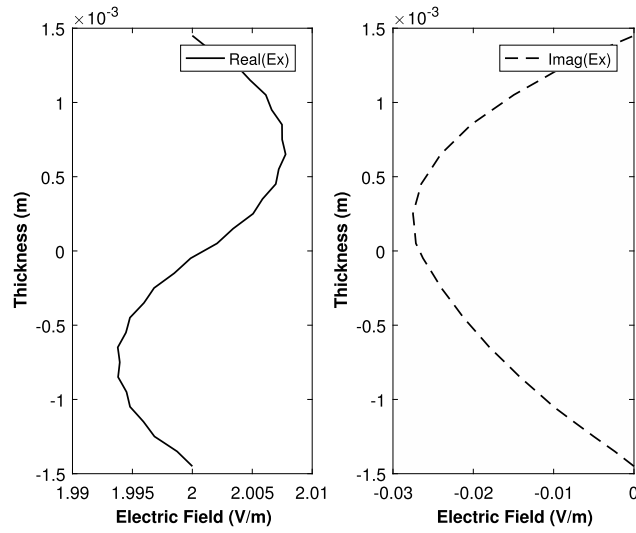
Fig. 16. Electrical field along the plate thickness, E_x(0.25, 0.25, z) .
