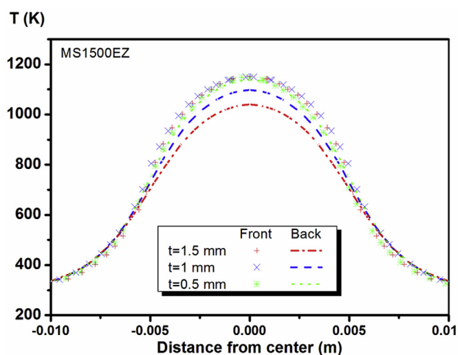
Fig. 9. Spatial distribution of temperature on the irradiated front and back surface of sheets with different thicknesses. The temperature was modelled for a square laser spot of 1 \text{ cm}^2 and scanning rate of 10 \text{ mm/s} .
