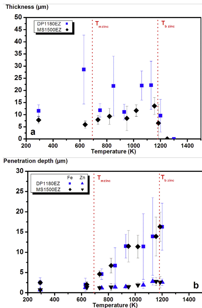
Fig. 8. a) Coating thickness and b) diffusion of zinc in the matrix and iron in the coating after laser treatment at a given temperature.
