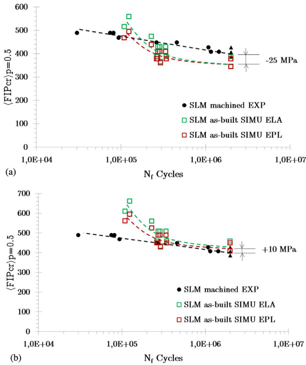
Fig. 23. Master Curve build for SVE obtained from profilometric analysis (a) and tomographic analysis (b).
