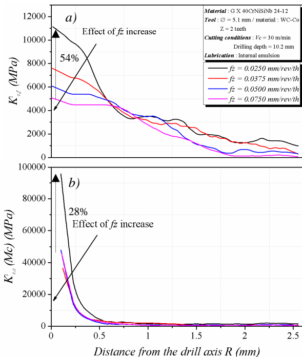
Fig. 5. (a) Specific cutting forces distribution in the feed direction K_{c,f}^l , and (b) the cutting direction K_{c,c}^l (b).
