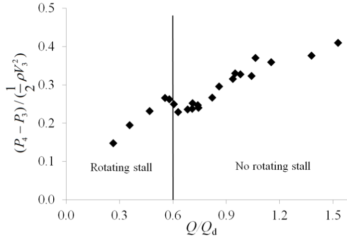
Figure 7 Diffuser static pressure recovery versus flow rate ratio
