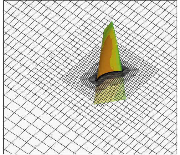
(b) Initial mesh S_0 .
