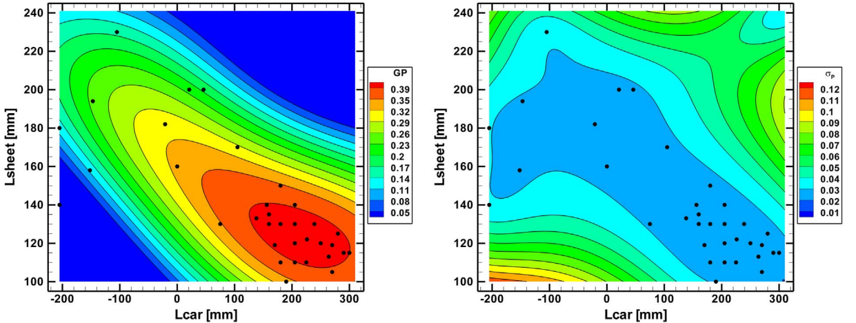
(a) GP model expectation.
