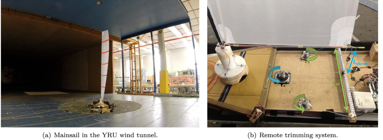
Fig. 3. Experimental setup.
