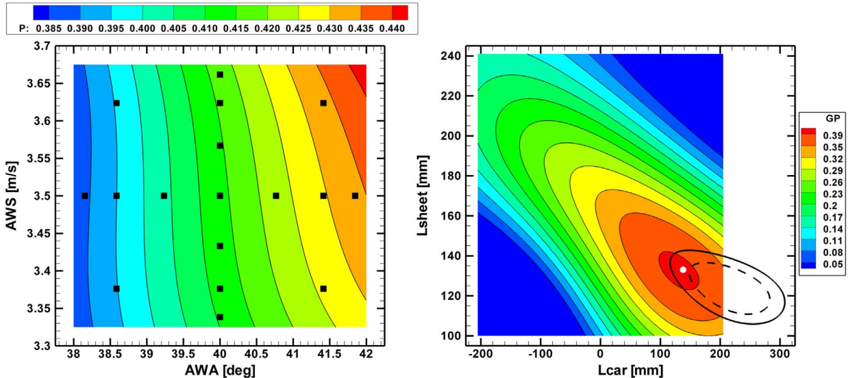
(a) Color contours of the PC approximation of the dependences of \mathcal{P}^{\text{num}}(\mathbf{x}_n) with the AWA and AWS. The dark points indicate the sparse grid points supporting the PC approximation. (b) Color contours of \hat{\mathcal{P}}_n^{\text{exp}}(\mathbf{x}) superposed with the boundaries of the uncertainty sets X(\sigma_{\mathcal{P}}) (dashed line) and X(\delta_{\text{max}}) (solid line) and experimental optimum (white point).
