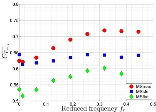
Figure 4: Evolution of the mean value of the optimization function with the reduced frequency for the different mainsails. AWA = 40^\circ , A=10\text{mm} .
