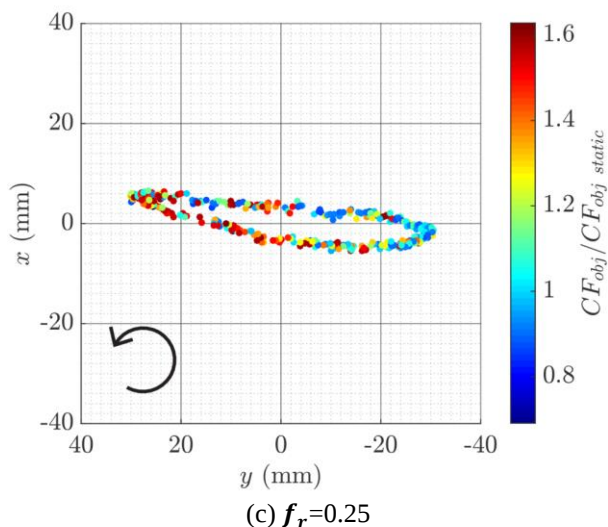
Figure 6: Mast head trajectory (above view also called “bird’s eye view”), AWA = 60° , A = 20mm , maximum camber mainsail. The colorbar represents the ratio of the instantaneous optimization target function over the optimization target function in static trim. x=y=0\text{mm} represents the static equilibrium position with no periodic forcing. The thick arrow on Fig. 6(a) shows the Apparent Wind Direction.
