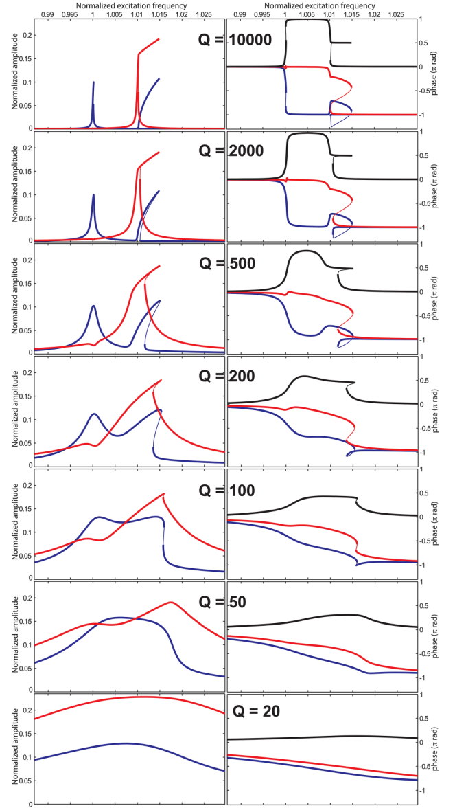
FIG. 7. Evolution of the elliptical transition as the quality factor decreases. The frequency difference is set to 1% and the excitation is increased to have QF = \text{constant} .
