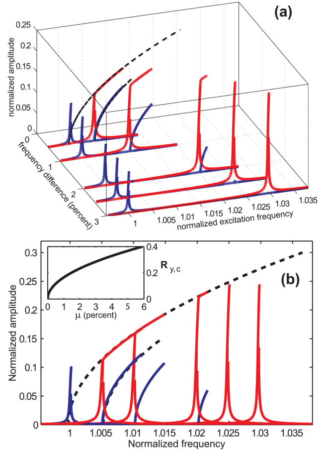
FIG. 3. Simulations showing the evolution of the elliptical transition as a function of the frequency difference between the polarizations. The simulations correspond to frequency differences of 0.5%, 1%, 2%, 2.5%, and 3%. The black dashed lines trace the backbone curves corresponding to the elliptical regime for \mu = 0.5\% following Eqs. (14) and (15). (a) 3 dimensional representation of the different response curves. (b) Projection of the response curves showing that the different transitions are well fitted by the backbone curve. Inset: Evolution of the critical amplitude, R_{y,c} , versus the frequency difference, \mu .
