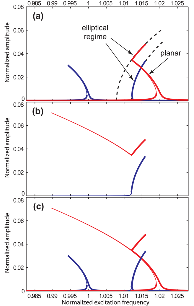
FIG. 6. Characterization of the elliptical transition for the second mode. (a) Frequency response of the polarizations showing soft spring Duffing behavior. Once again, for the higher polarization, the elliptical regime is observed with hard spring behavior. The dashed lines present the analytical backbone curves for the elliptical regime [Eqs. (14) and (15)]. (b) New isolated set of solutions corresponding to the elliptical regime. (c) Superposition of the two sets of solutions.
