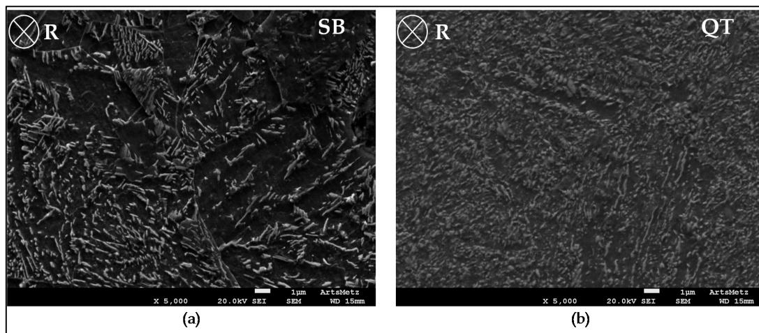
Figure 3. SEM microscopy for pre-machined bars ( \times 5000 ) (a) SB and (b) QT.
