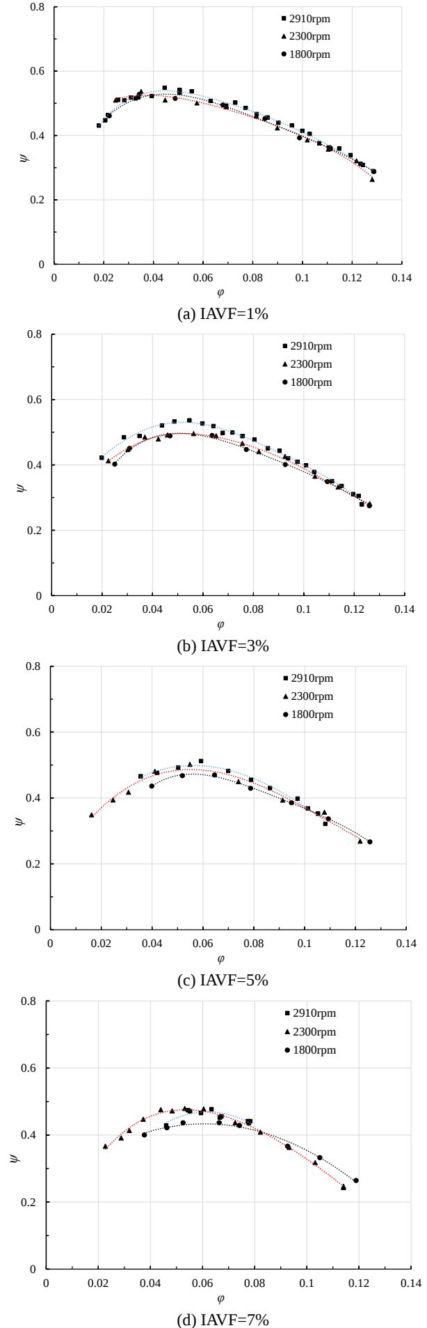
Figure 6. Pump head coefficients comparison at different IAVF
