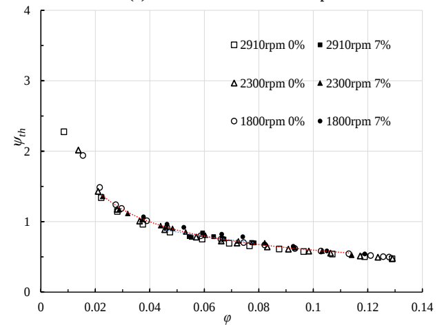
Fig.5. Pump performance curves under two phase flow conditions
