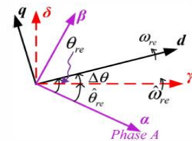
Fig 1. \alpha - \beta stationary frame, d_1 - q_1 rotating frame, \delta - \gamma estimated frame [2]
