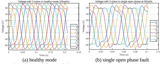
Fig. 13. Voltage per phase with 3-rotor
