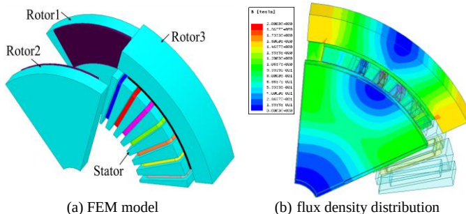
Fig. 5 One-sixth of the structure of the proposed AFPM
