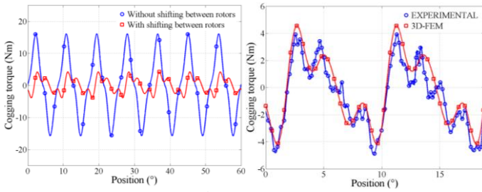
(a) FEM results with/without shifting (b) experimental validation Fig. 9. Cogging torque characteristics with conventional 2-rotor AFPM
