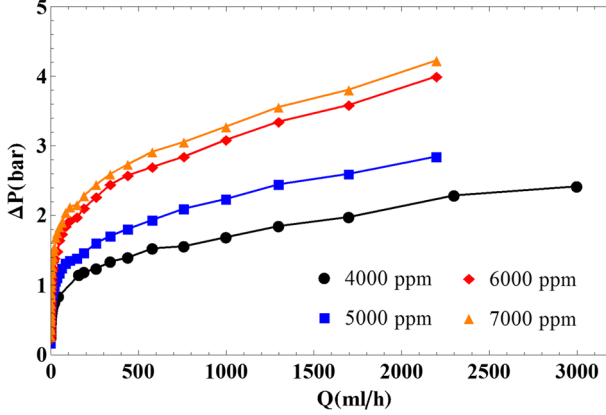
Fig. 7 ( Q_i, \Delta P_i ) raw data obtained from injection of xanthan gum solutions with different polymer concentrations through analogous samples of A10 sintered silicate
