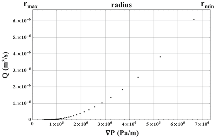
Fig. 2 ( Q_i, \nabla P_i ) data corresponding to the numerical injection of a Herschel–Bulkley fluid with \tau_0 = 10 Pa, k = 1 Pa s n and n = 0.60 through a bundle of 1,000,000 capillaries whose radii are distributed according to the original p(r) . The upper axis represents the radii of the pores joining the flow at each \nabla P (smaller pores at higher \nabla P )
