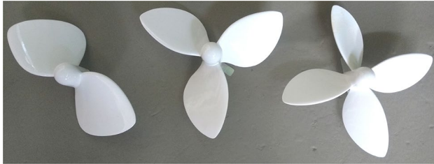
Fig. 6 Small-scale runners with two, three and four blades
