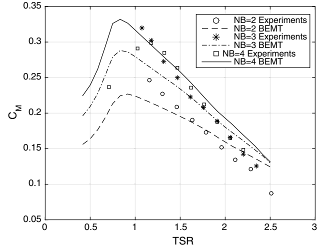
Fig. 16 Torque coefficient for BEMT simulations and experiments
