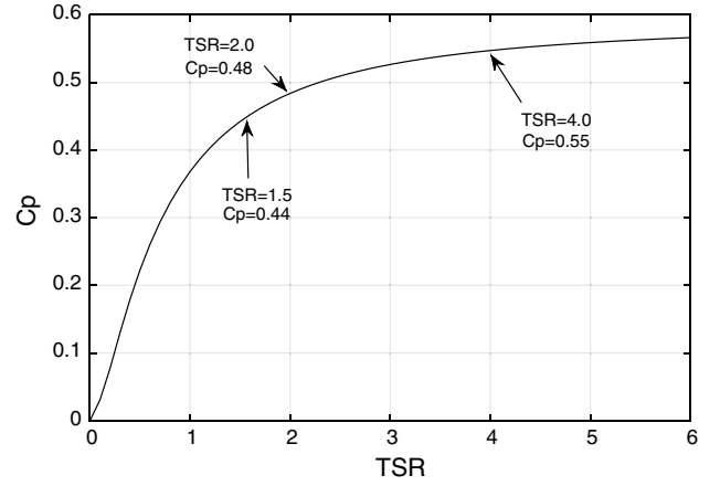
Fig. 9 Optimum Glauert power coefficient—infinite number of blades
