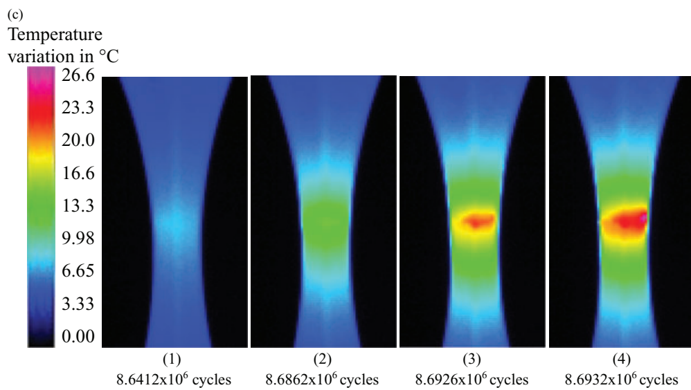
Fig. 3 Evolution of the temperature variation for the AlSi7 Mg06 alloy.
