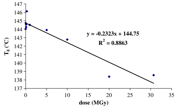
Fig. 6. Decrease of glass transition temperature with irradiation dose for 60 \mu\text{m} thick amorphous films.
