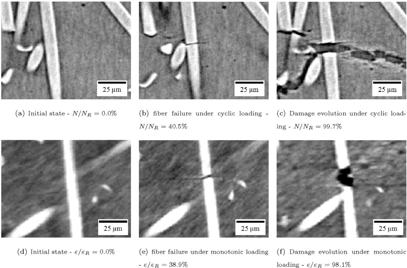
Fig. 9. Fiber failure evolution according to the loading.
