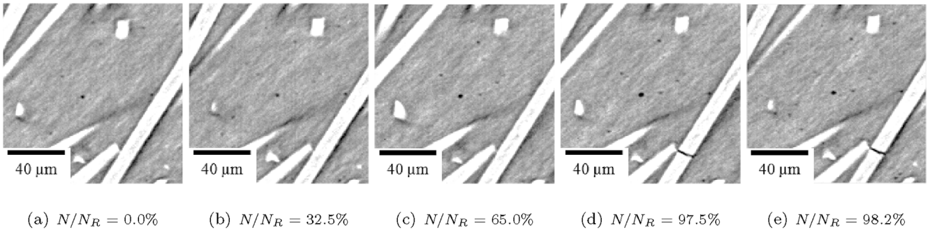
Fig. 4. Cavitation - RH50 45° specimen N_R = 1537 cycles.
