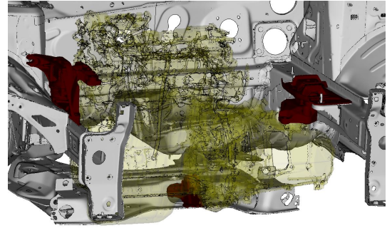
Figure 12: Assembled powertrain unit and its suspension
