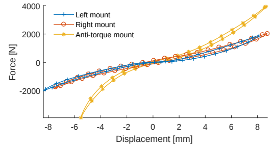
Figure 8: Force/displacement response for the three tested mounts
