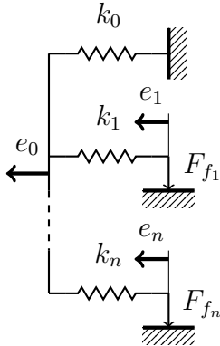
Figure 5: Rheologic scheme for Iwan's model
