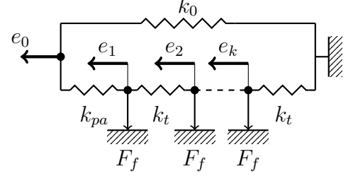
Figure 7: Rheologic scheme for the STS model
