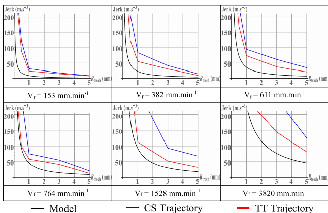
— Model — CS Trajectory — TT Trajectory Fig. 11. Maximum jerk function of R_{\text{troch}} for different feed rates.
