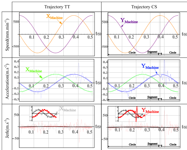
— Model - - - - Nominal ····· Effective Fig. 10. Dynamic of the axis machine during trochoidal milling for V_f = 764 \text{ mm}\cdot\text{min}^{-1} .
