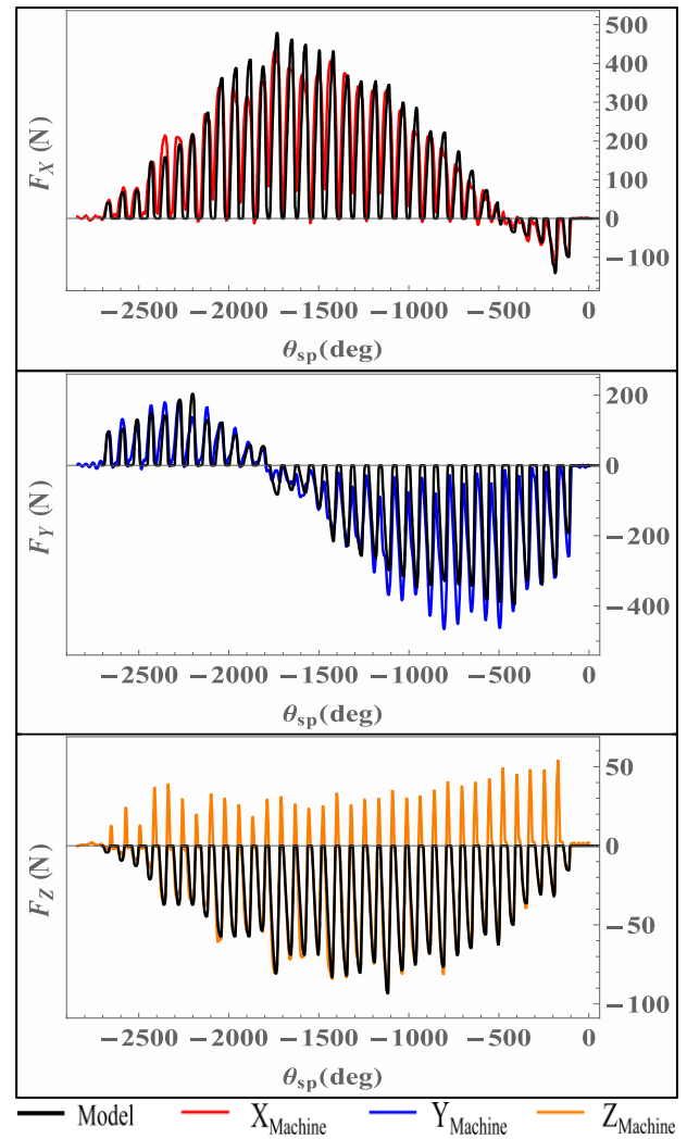
Fig. 9. Cutting forces modelled and measured in down milling ( V_c = 60 \text{ m.min}^{-1} , f_z = 0.1 \text{ mm.rev}^{-1}.\text{tooth}^{-1} , a_p = 5 \text{ mm} , R_{troch} = 1 \text{ mm} , P_{troch} = 0.05 \text{ mm} ).
