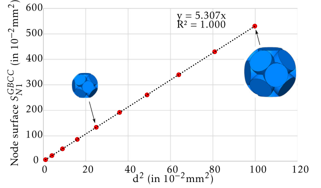
Fig. 6. Surface regression of the GBCC lattice first node geometry.
