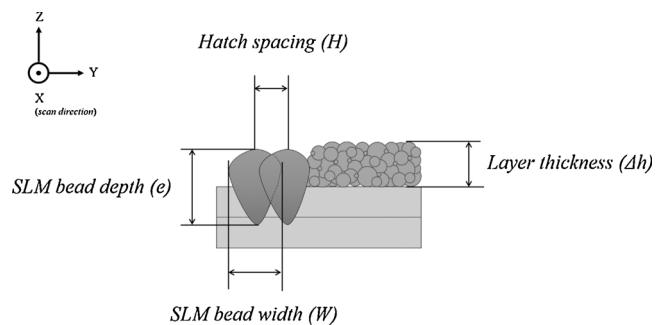
Fig. 2. Illustration of the key dimensions to estimate the formation of LOF, according to [22].
