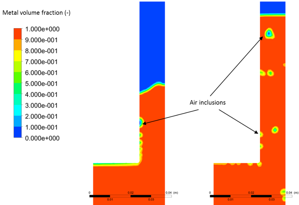
Figure 11 : Observation of simulated air pockets entrapped in the metal at two instants after the section restriction in “Case C”
