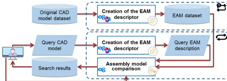
Fig. 2. Assembly retrieval framework.
