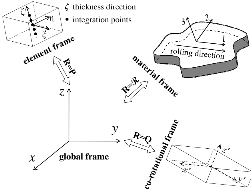
Figure 2. Illustration of the local coordinate systems, and the associated rotation matrices, used in the formulation of SHB-EXP solid-shell elements
