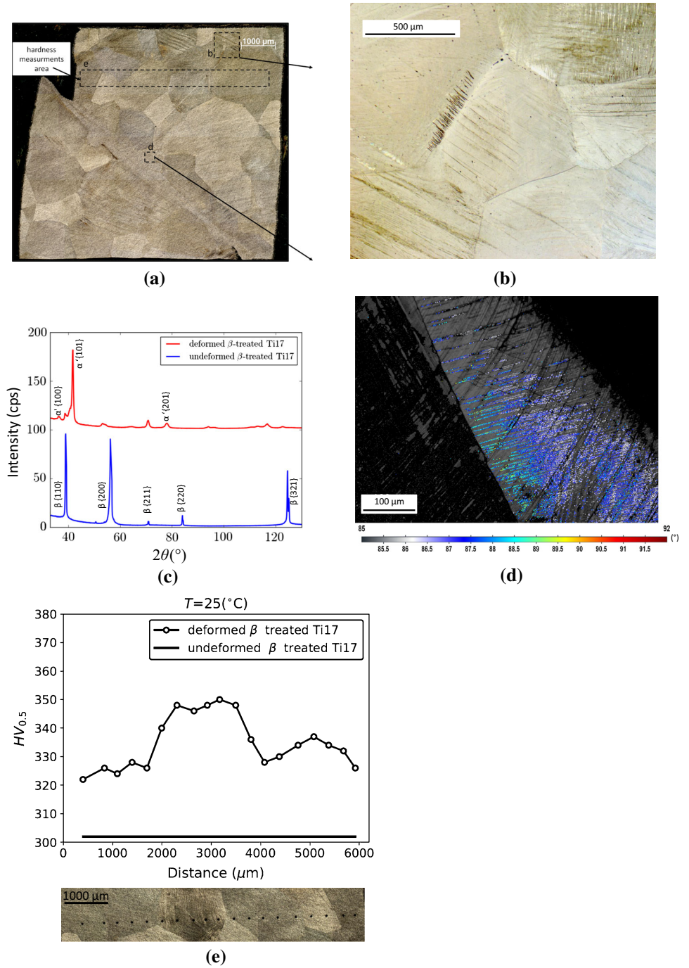
Figure 13 a Metallographic observation of an adiabatic shear band in a deformed \beta -treated Ti17 specimen at a strain rate of 10 \text{ s}^{-1} and a temperature of 25^\circ\text{C} . b \alpha' martensite. c XRD pattern obtained with a Cu K\alpha radiation. d Observation of a \{10\bar{1}2\}\langle\bar{1}011\rangle extension twin in a martensitic domain in a \beta -treated Ti17 specimen that has been deformed at 25^\circ\text{C} and 10 \text{ s}^{-1} . The Atex software [48] has been used for the post-processing of EBSD data. e Evolution of the final Vickers hardness on a line perpendicular to the compression axis.
