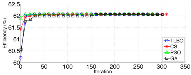
Fig. 13. Comparison of best fitness's variation with the iterations: case 1–scenario 2.
