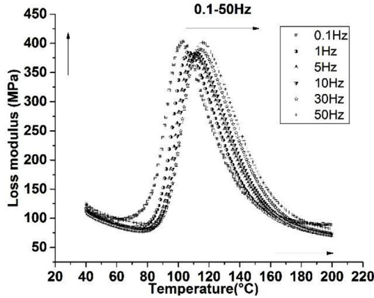
Fig. 6. Effect of frequency on loss modulus spectrum of PPS/GF composite in the range of 0.1 Hz–50 Hz.
